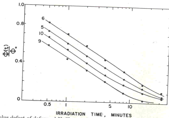
FIG. 5. Relative modulus defect of deformed NaCl crystals subjected to X-irradiation. Each curve is numbered with the identification number of the crystal measured. Data for crystal No. 4 superimposes on that for crystal No. 9.
