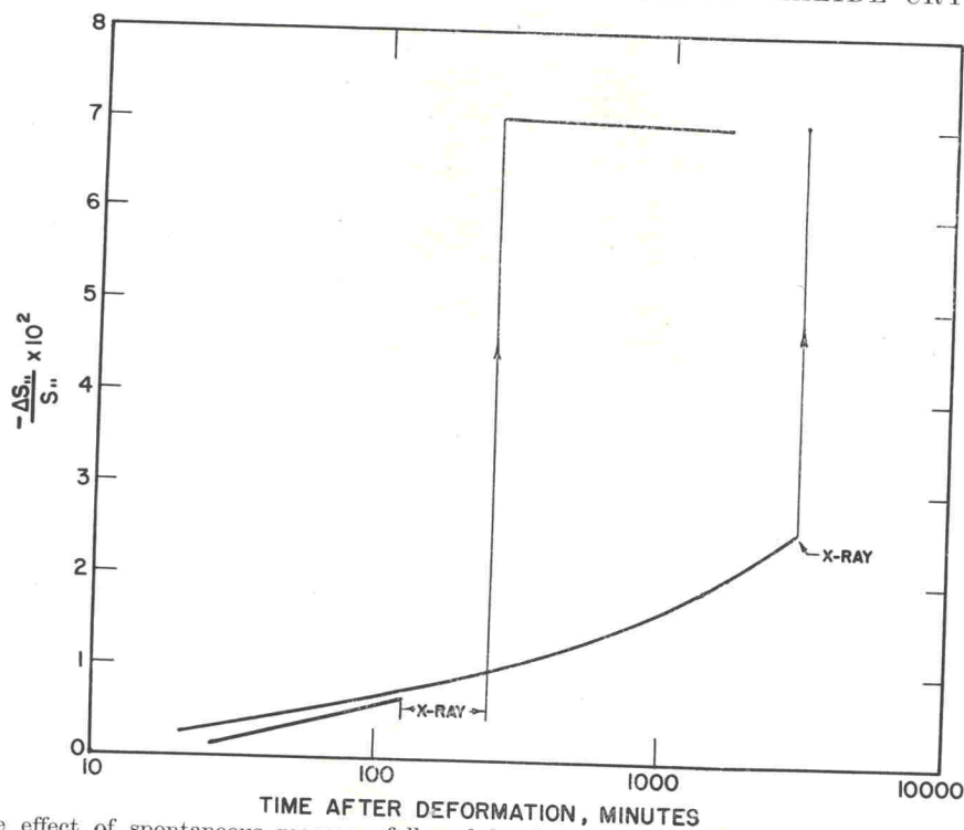
FIG. 4. The effect of spontaneous recovery followed by X-irradiation on the elastic constant of two crystals (Nos. 12 and 13). Specimens were subjected to X-irradiation for 2 h at the times indicated.
